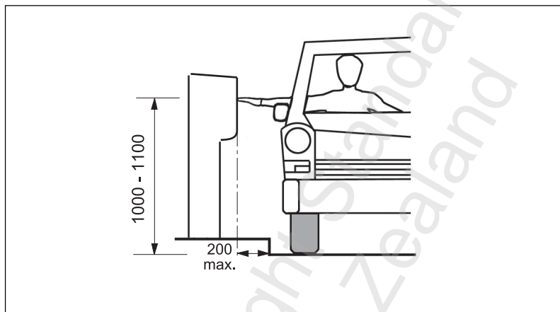
Figure 9 – Facilities accessible from vehicle
