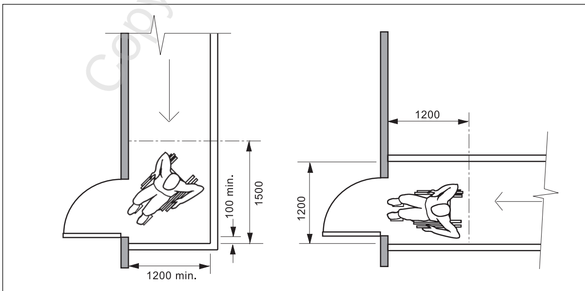
Figure 15 – Landings to inward opening doors
