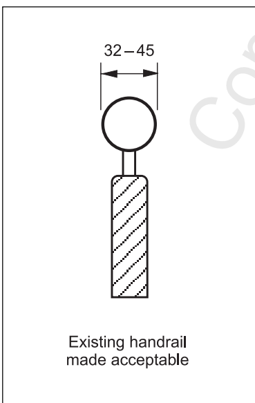
Figure C3 – Handrail adaptation
