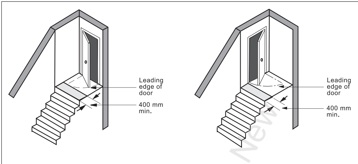
Figure 24 – Opening of doors
